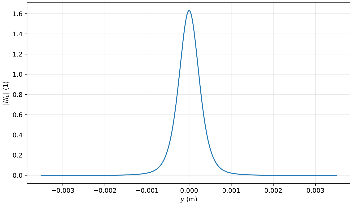
Intensity profile I(x=0, y, z=1.990)/I_0 , P_{in}=0.9P_{cr} , artificial time
